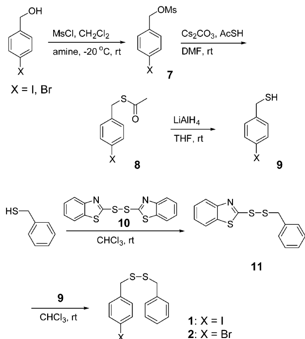
Figure 2. Synthetic pathway of benzyl 4-halobenzyl disulfide ( 1 and 2 ).
