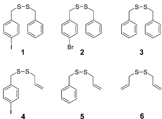
Figure 1. Structures of disulfides: benzyl 4-iodobenzyl disulfide ( 1 ), benzyl 4-bromobenzyl disulfide ( 2 ), dibenzyl disulfide ( 3 ), allyl 4-iodobenzyl disulfide ( 4 ), allyl benzyl disulfide ( 5 ) and diallyl disulfide ( 6 ).
