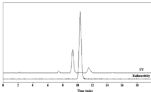
Figure 6. Semipreparative HPLC traces of [^{123}\text{I}/^{125}\text{I}]\mathbf{1} . HPLC solvents: 85:15 \text{CH}_3\text{OH}-\text{H}_2\text{O} ; HPLC column: C18 silica gel; t_R = 10.4 min; flow rate: 4 mL/min; UV detector (UV) and a NaI(Tl) radioactivity detector.
