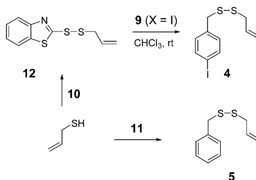
Figure 3. Synthetic pathways of allyl 4-iodobenzyl disulfide ( 4 ) and allyl benzyl disulfide ( 5 ).
