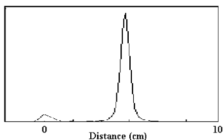
Figure 5. Radio-TLC of the radioiodination mixture. Developing solvents: 49:1 hexane–ethyl acetate.
