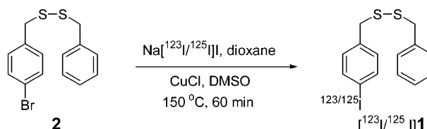
Figure 4. Synthetic pathway of [ ^{123}\text{I}/^{125}\text{I} ] 1 .
